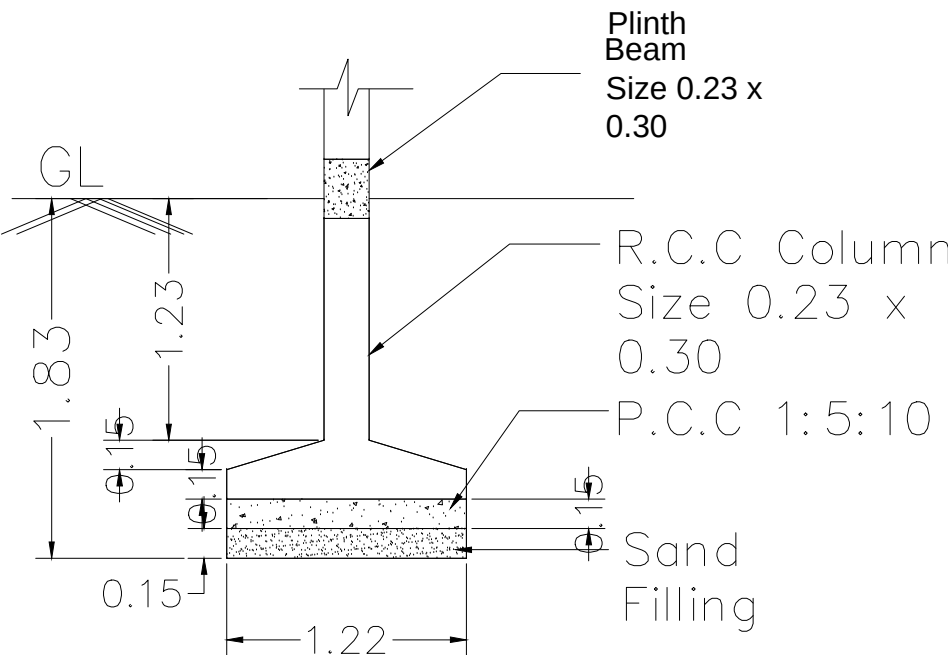
FOUNDATION DETAILS
