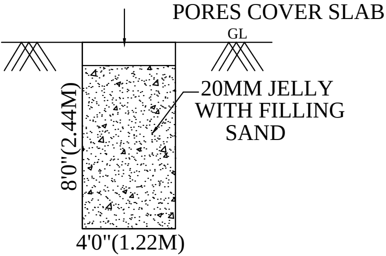
RAINWATER HARVESTING UNIT
