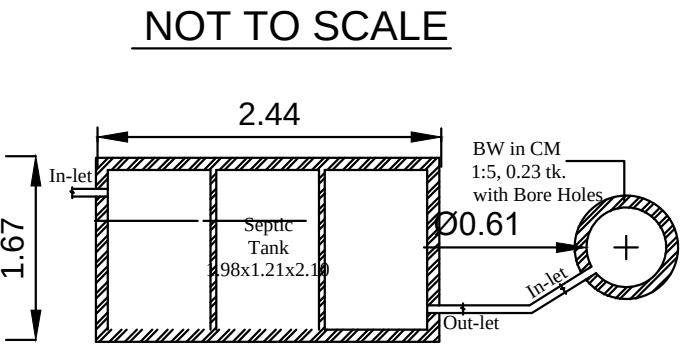
PLAN - SEPTIC TANK & SOAK PIT
