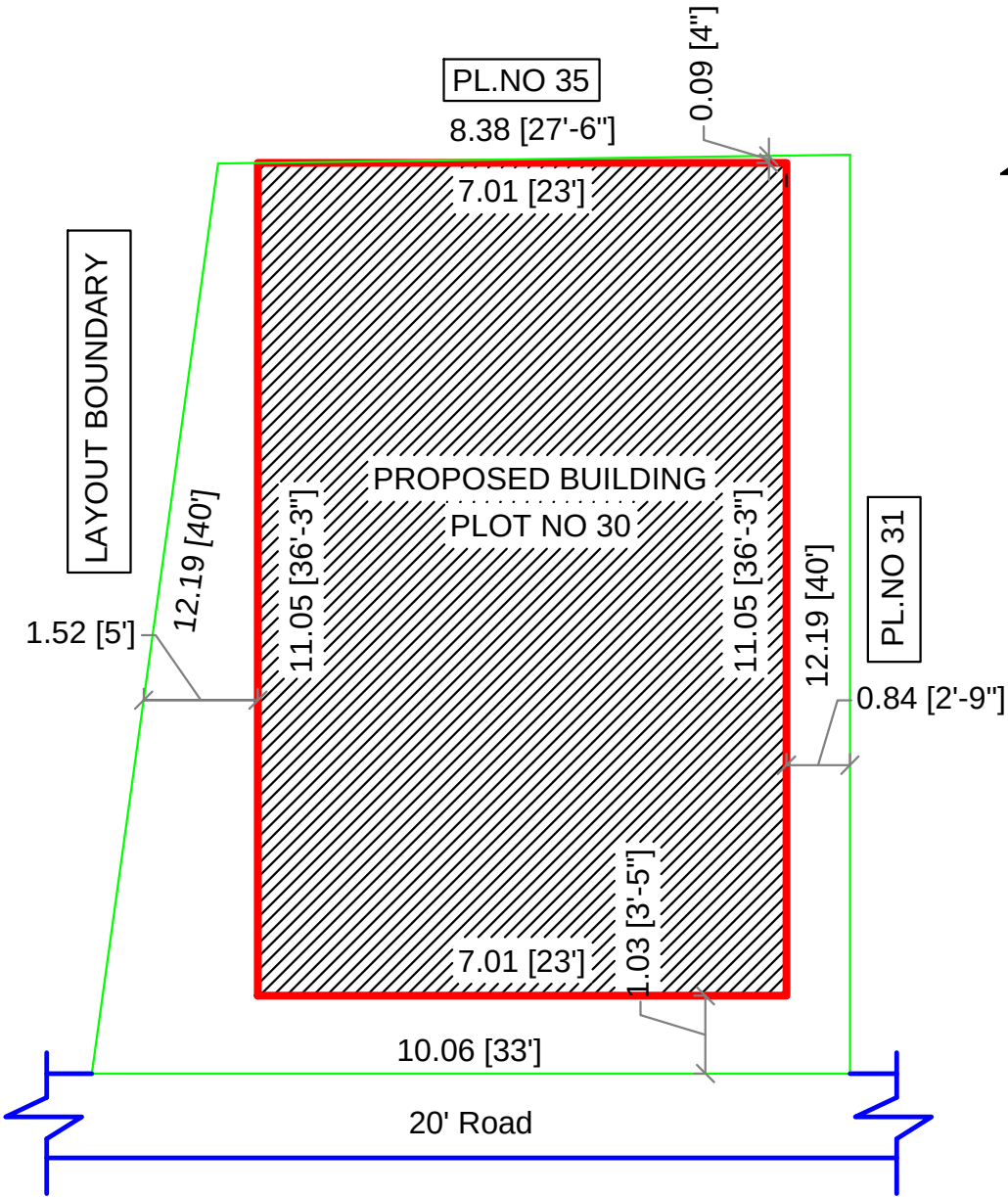
SITE PLAN (1:100)
