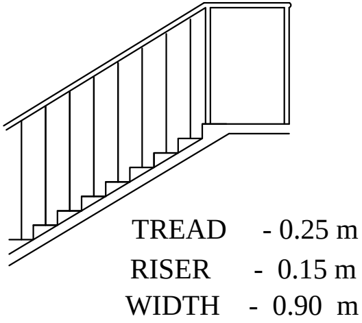
STAIRCASE DETAILS
