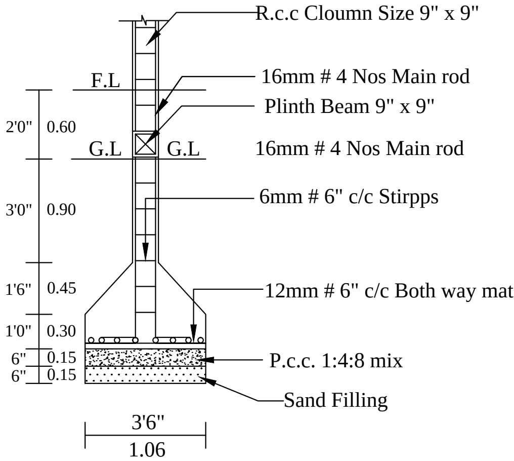
COLUMN DETIAL
