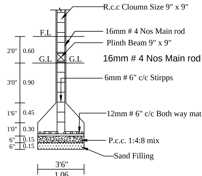
COLUMN DETIAL
