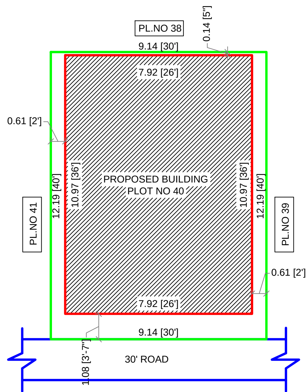
SITE PLAN (1:100)
