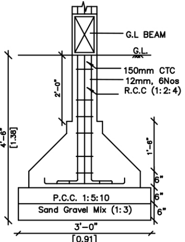
R.C.C. COLUMN FOOTING DETAILS SCALE : 1:25
