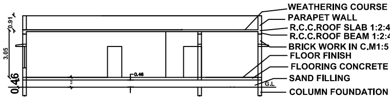
SECTION- SS
