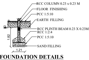
FOUNDATION DETAILS
