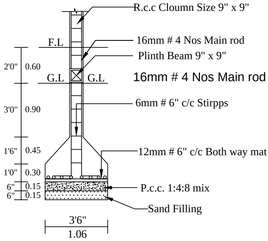
COLUMN DETIAL
