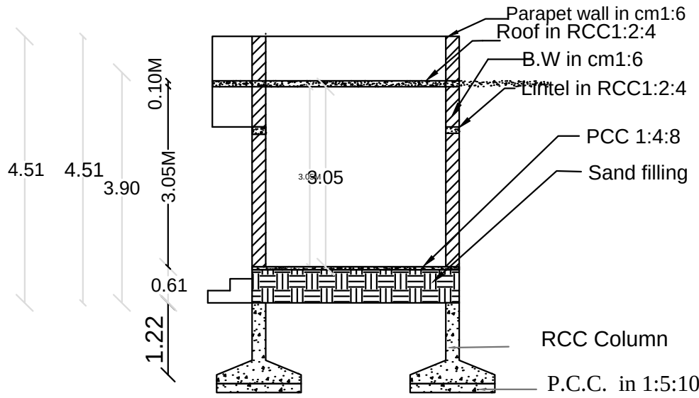
SECTION PLAN SHOP -2
