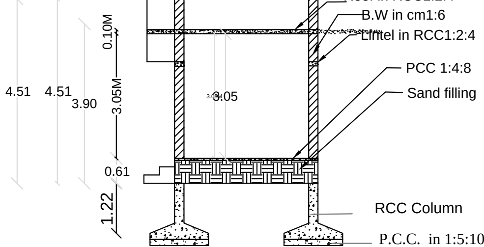
SECTION PLAN SHOP -1
