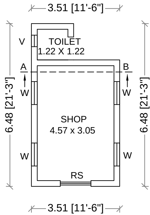
GROUND FLOOR PLAN SHOP -1
