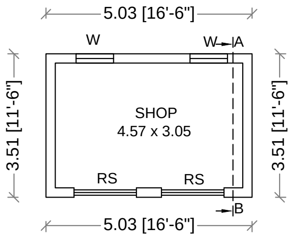
GROUND FLOOR PLAN SHOP -2
