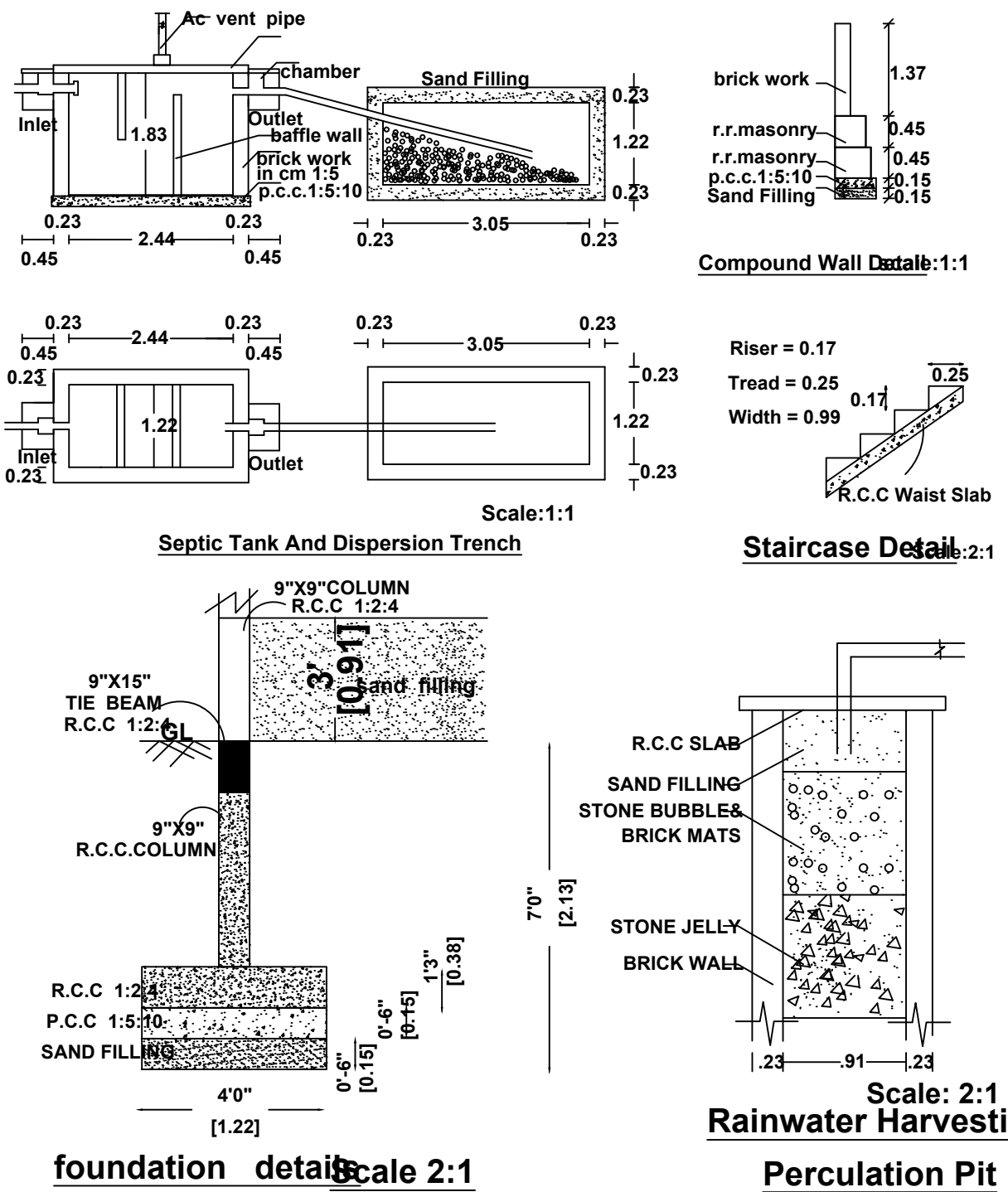
foundation details
