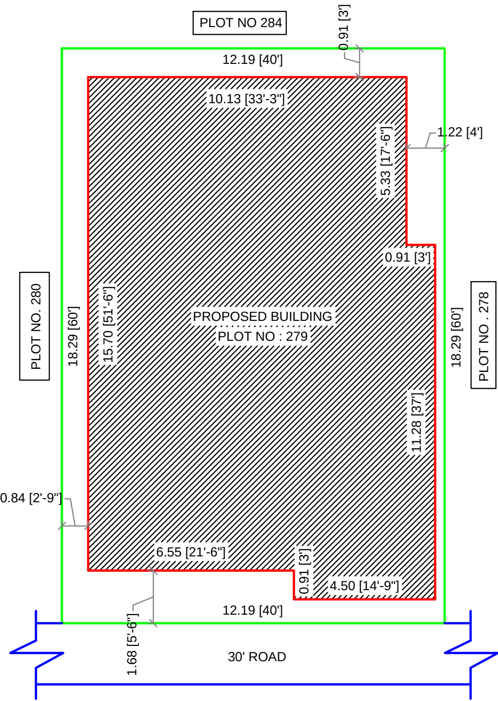
SITE PLAN (1:100)
