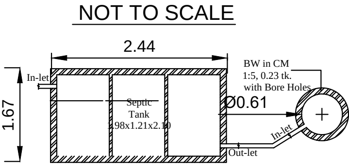
PLAN - SEPTIC TANK & SOAK PIT
