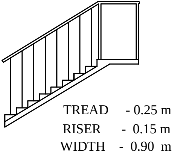
STAIRCASE DETAILS
