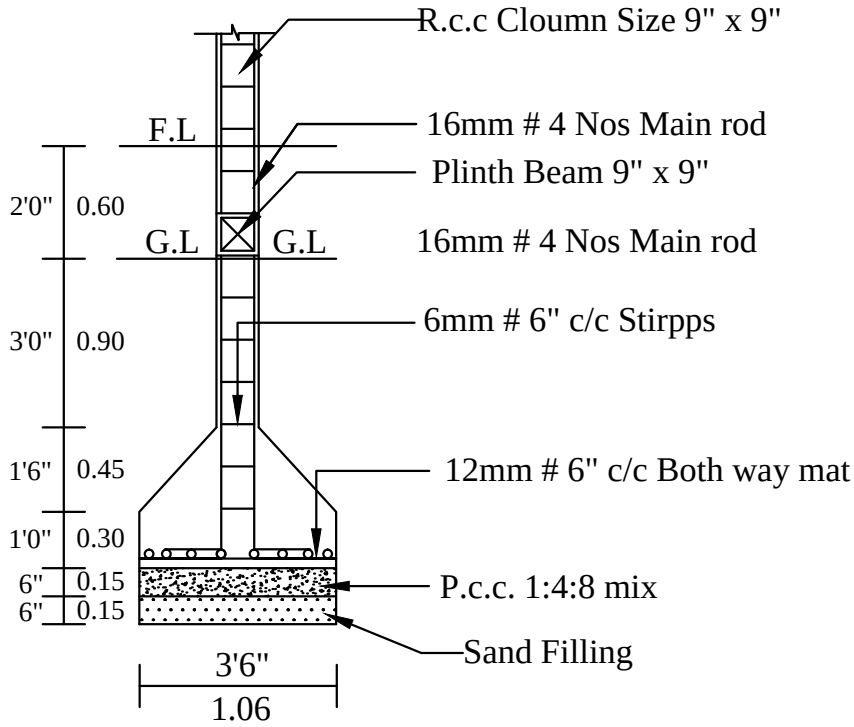
COLUMN DETIAL
