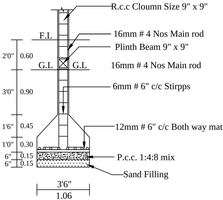
COLUMN DETIALS
