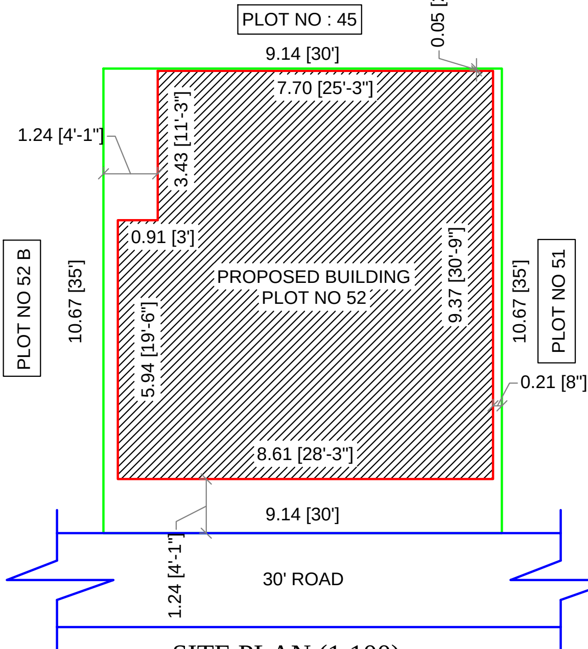
SITE PLAN (1:100)
