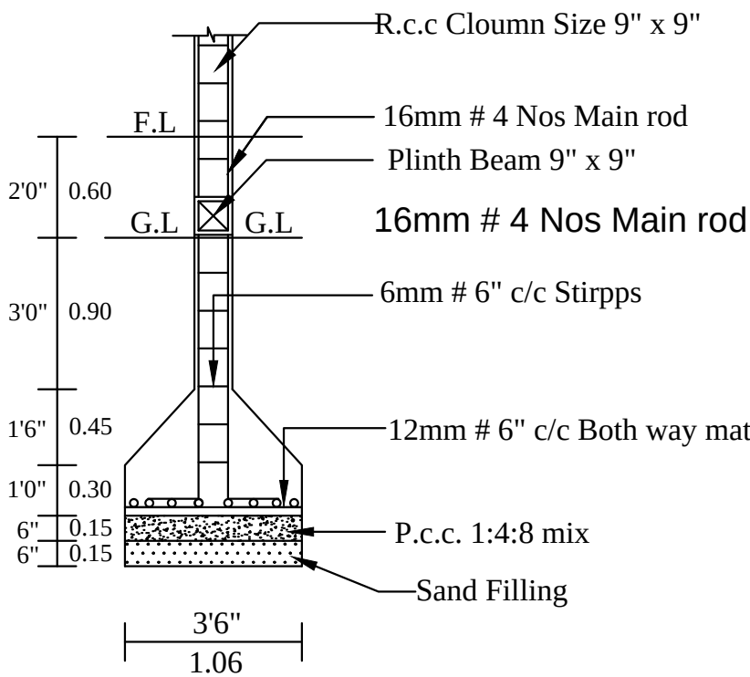
COLUMN DETIAL
