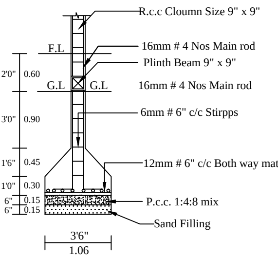
COLUMN DETIAL
