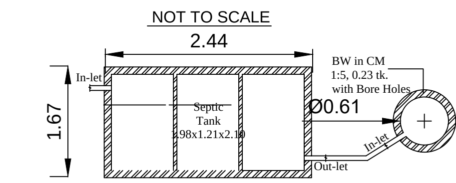
PLAN - SEPTIC TANK & SOAK PIT
