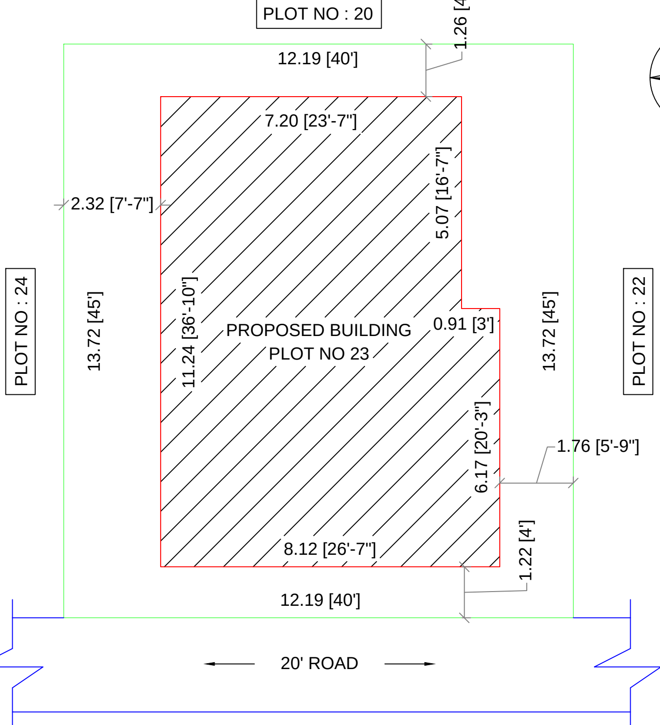
SITE PLAN (1:100)
