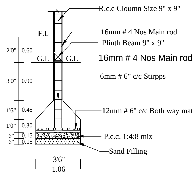
COLUMN DETIAL
