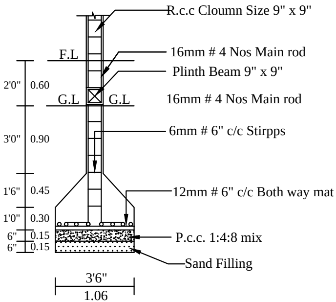
COLUMN DETAILS
