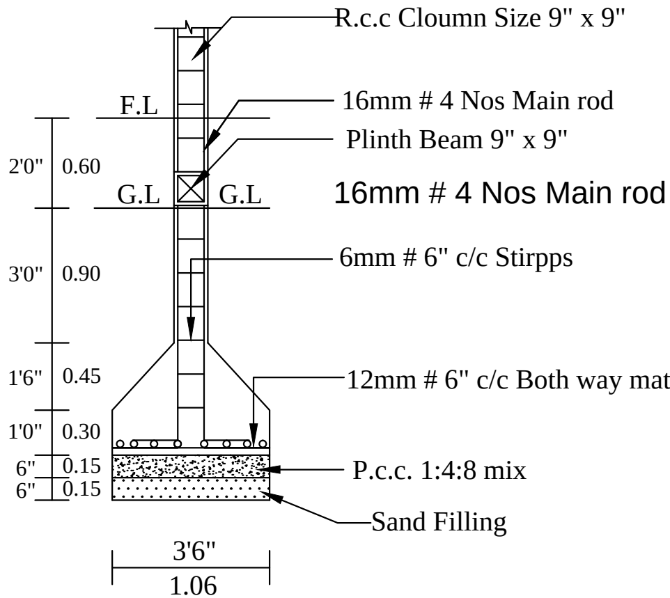
COLUMN DETIAL
