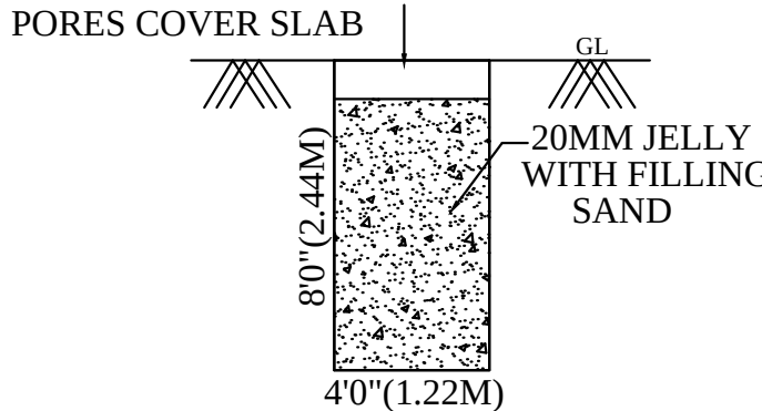
RAINWATER HARVESTING UNIT
