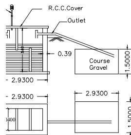
TANK & D-TRENCH DETAILS
