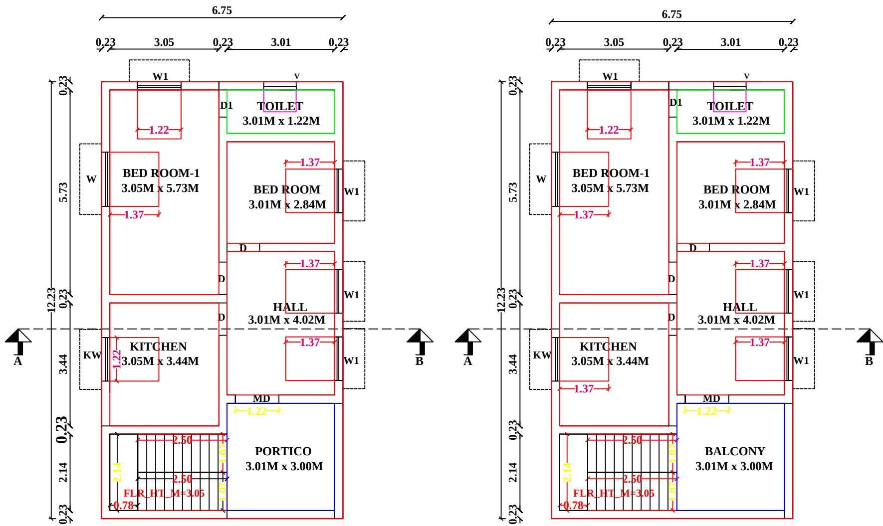
FLOOR-01 PRO-FIRST FLOOR PLAN
