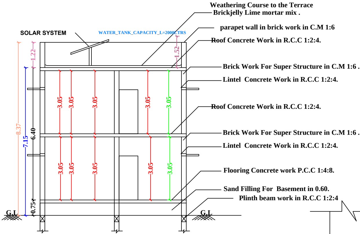
SECTION-AB
