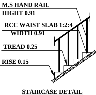
STAIRCASE DETAIL
