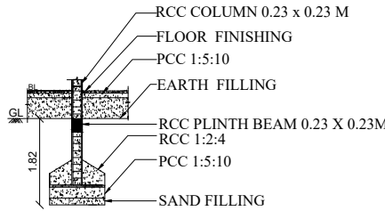
FOUNDATION DETAILS
