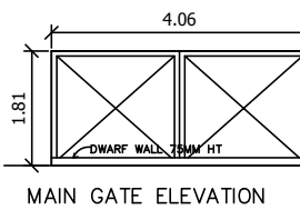
MAIN GATE ELEVATION
