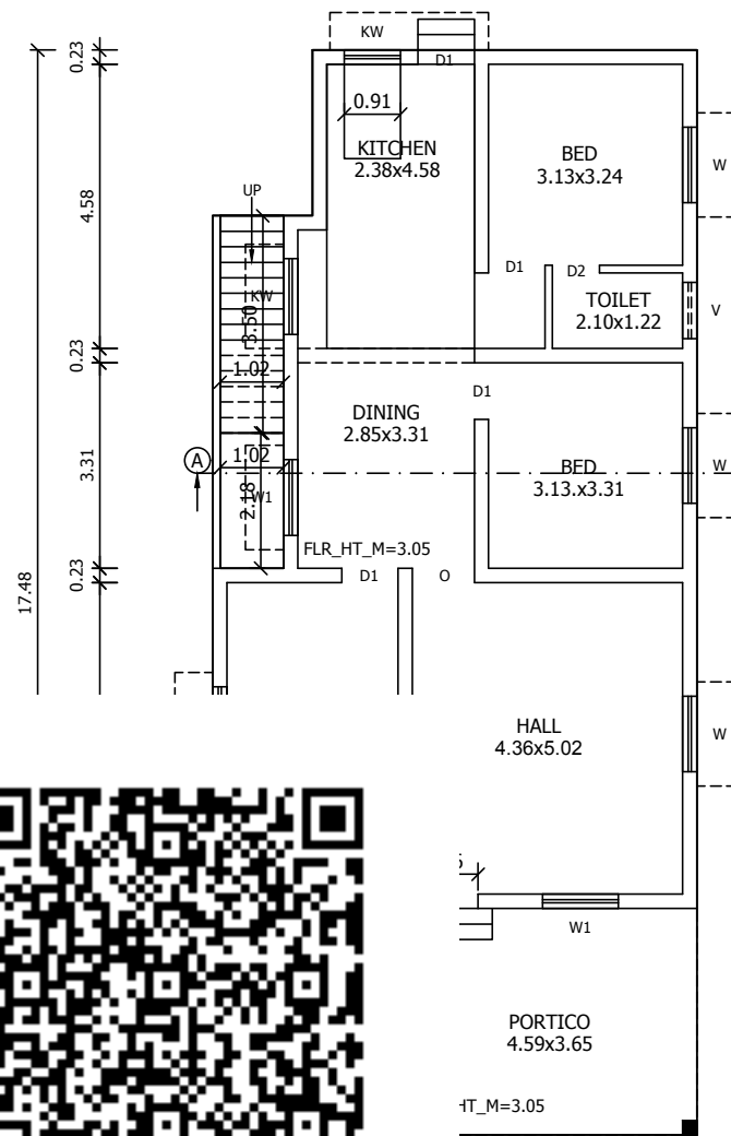
FLOOR PLAN
