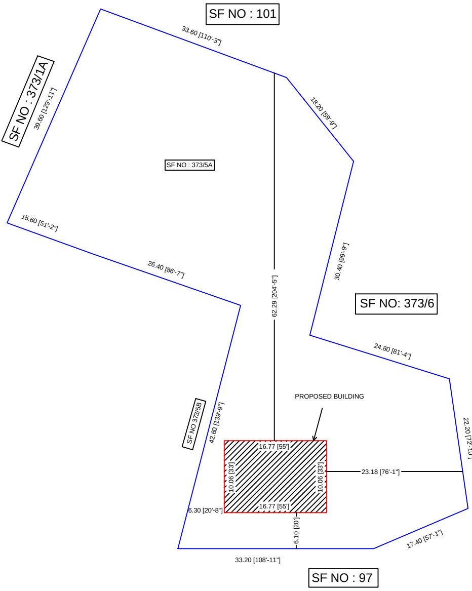
SITE PLAN
