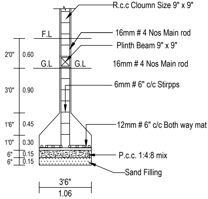
COLUMN DETIAL
