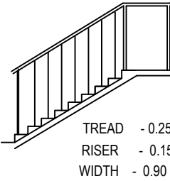
STAIRCASE DETAILS
