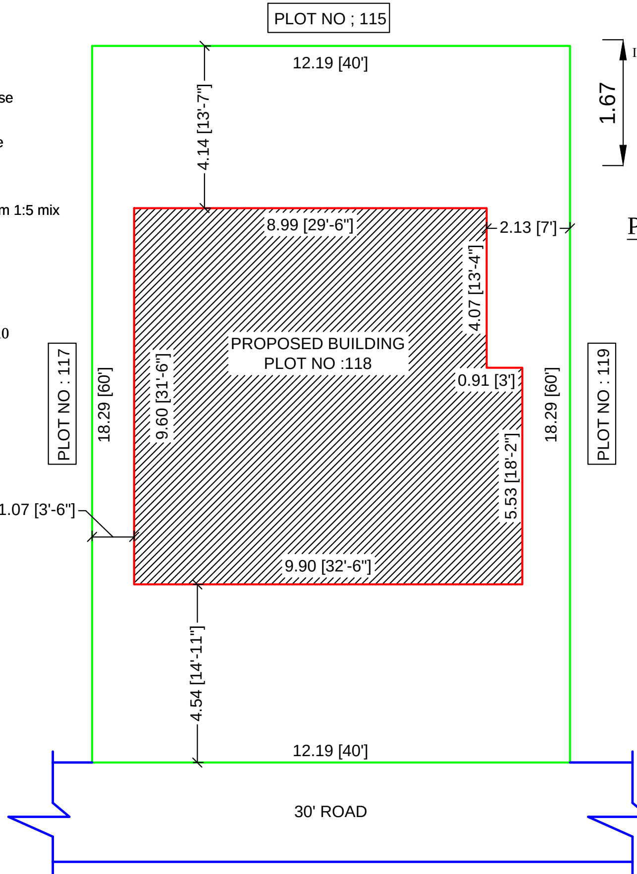
SITE PLAN (1:100)
