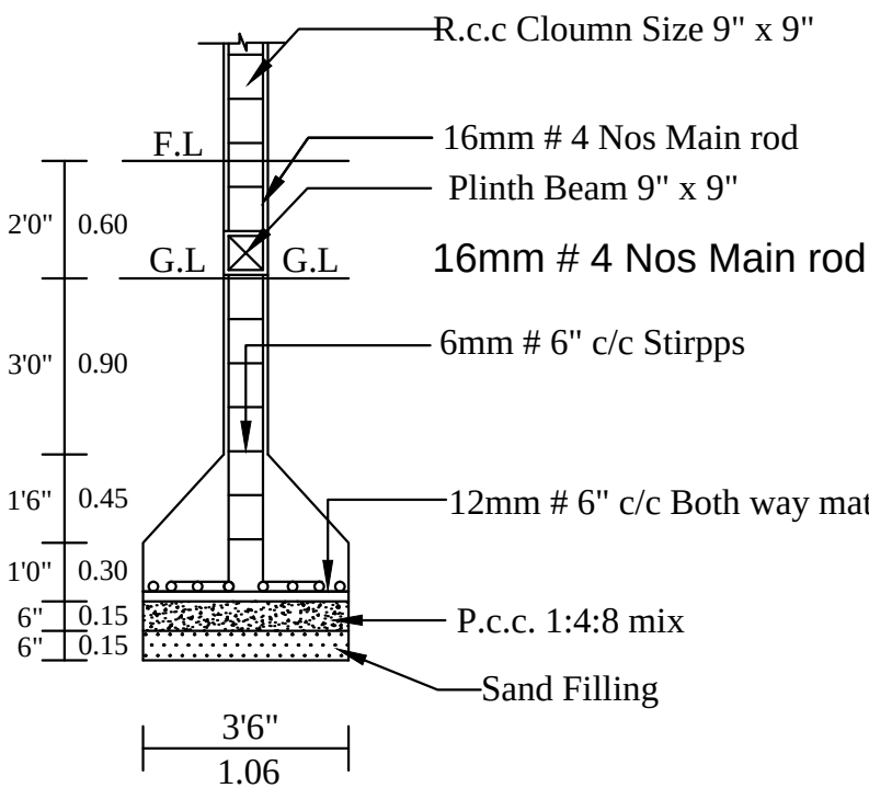
COLUMN DETIAL
