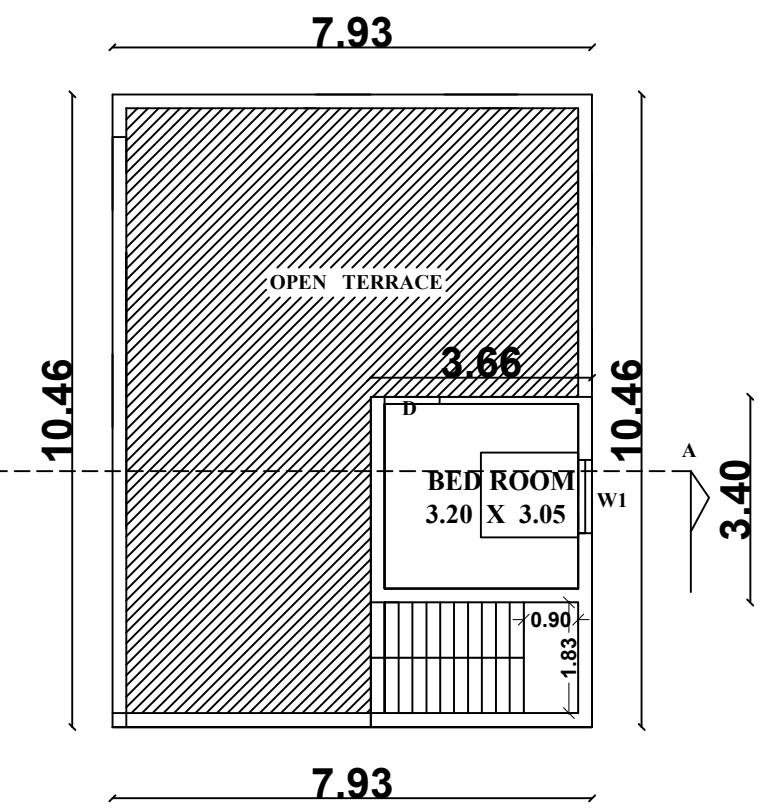
FLOOR- FIRST
