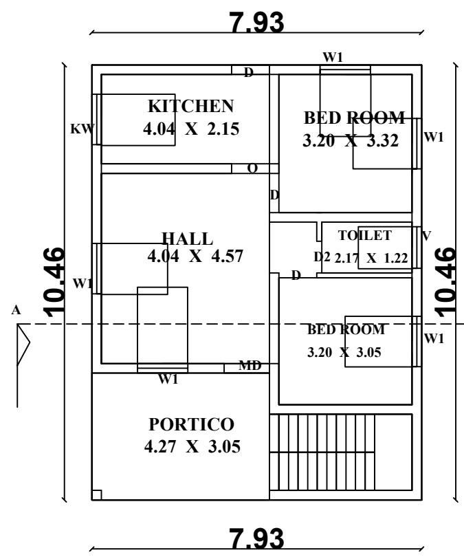
FLOOR- GROUND
