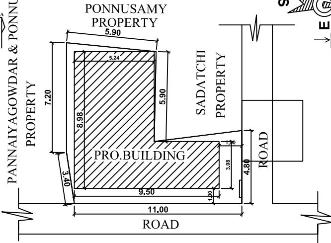
SITE PLAN
