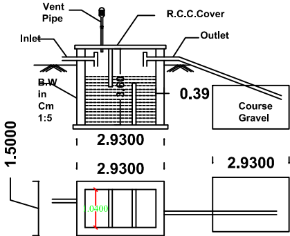
SEPTIC TANK & D-TRENCH DETAILS
