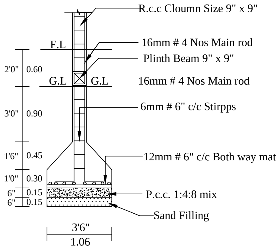
COLUMN DETIAL
