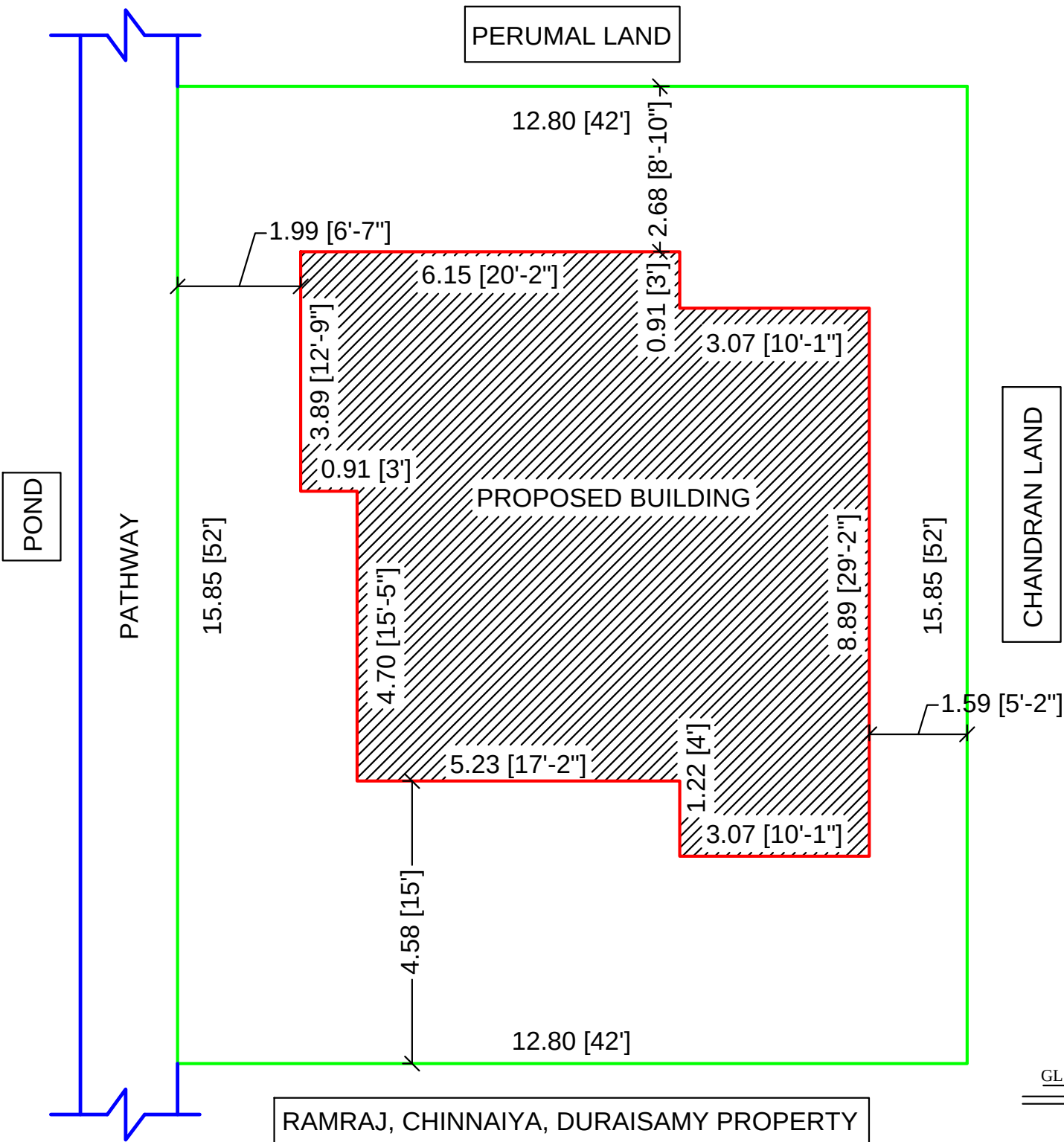
SITE PLAN (1:100)
