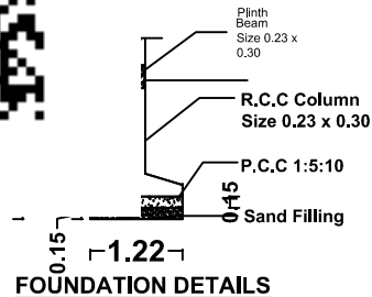
FOUNDATION DETAILS
