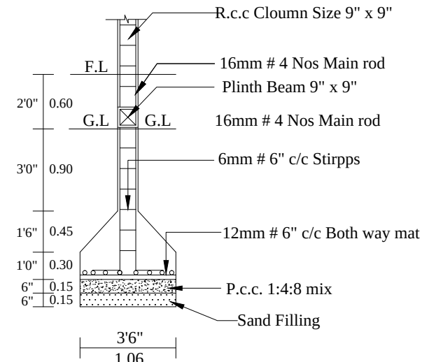
COLUMN DETAILS
