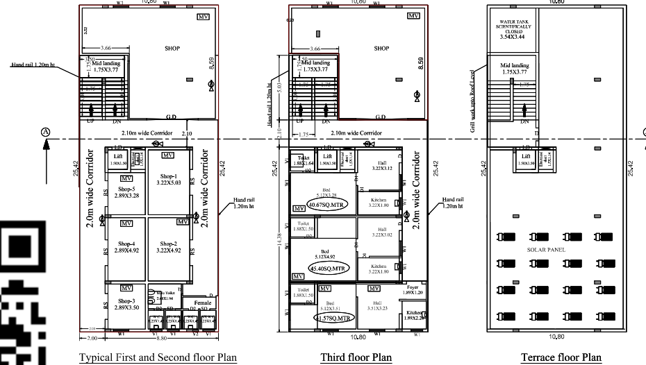
Typical First and Second floor Plan
