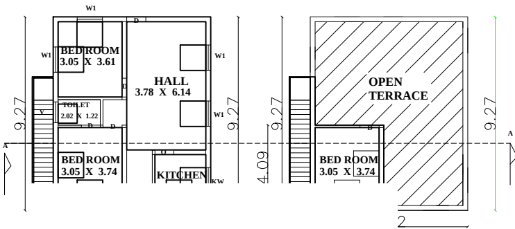
- FIRST RST FLOOR PLAN
