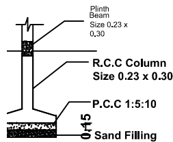
FOUNDATION DETAILS
