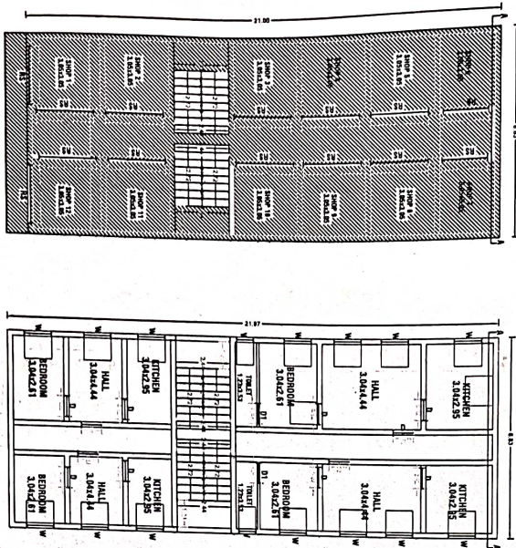
EXISTING, GROUND FLOOR PLAN PRO, FIRST FLOOR PLAN
