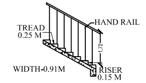
STAIRCASE DETAILS
