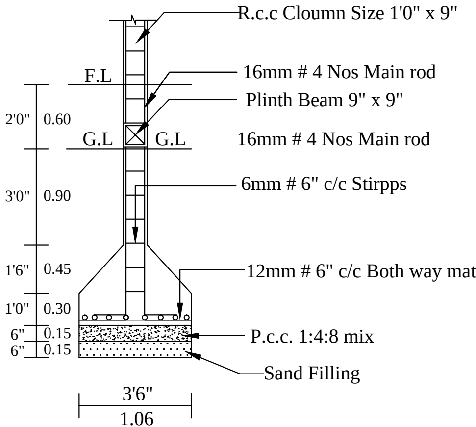
COLUMN DETIAL
