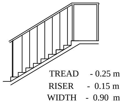
STAIRCASE DETAILS
