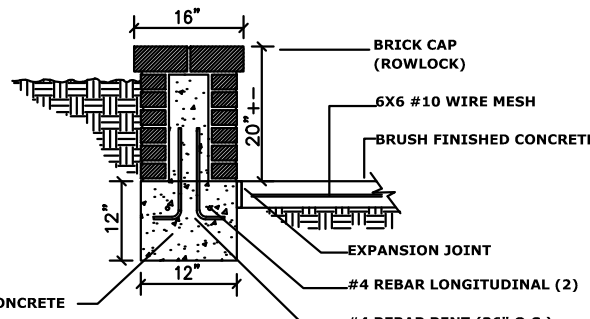
RAISED BRICK PLANTER
