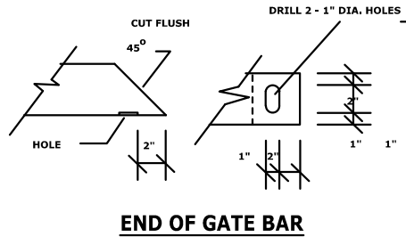
END OF GATE BAR
