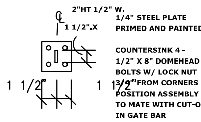
HASP ASSEMBLY
