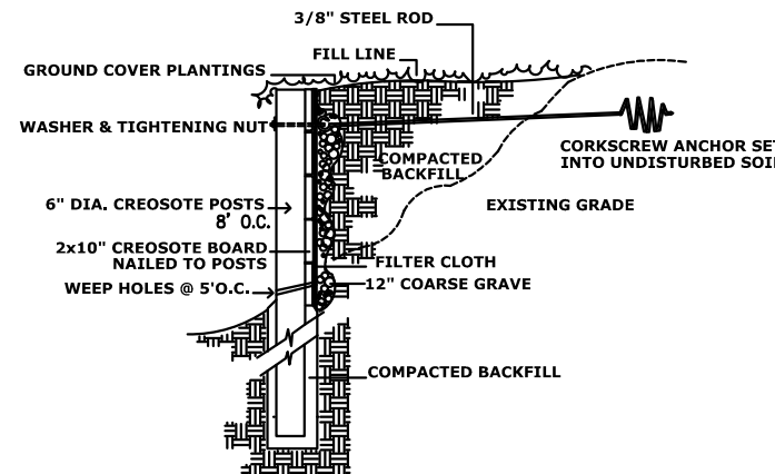
WOOD RETAINING WALL
