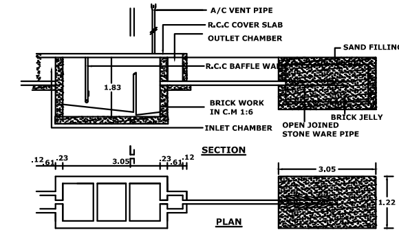
DETAILS OF SEPTIC TANK AND DISPERSION TRENCH
