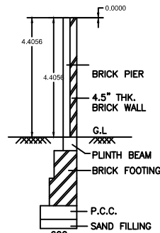
COMPOUND WALL
