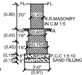
FOUNDATION DETAIL (NOT TO SCALE)
