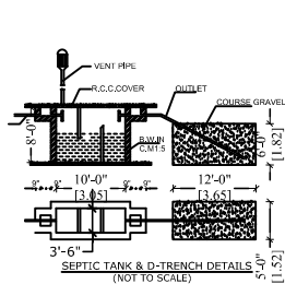
SEPTIC TANK & D-TRENCH DETAILS (NOT TO SCALE)
