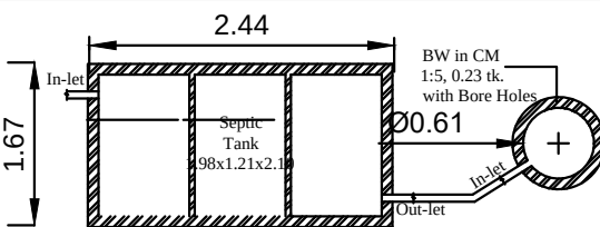
SECTION - SEPTIC TANK & SOAK PIT
