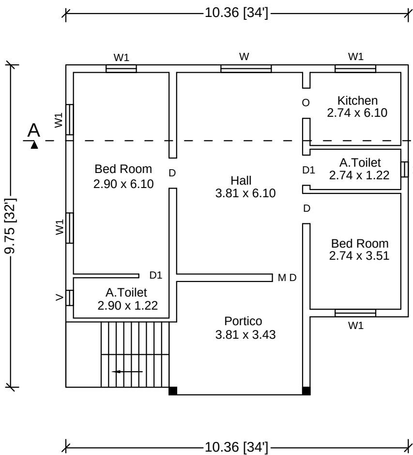
EXG. GROUND FLOOR PLAN
