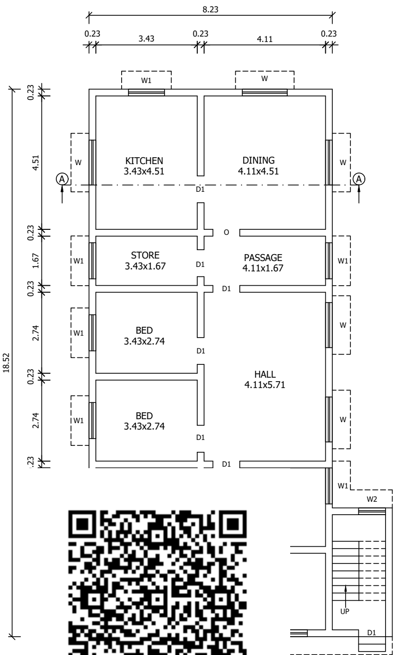
PLAN
