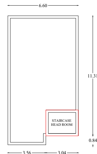
PROPOSED TERRACE FLOOR PLAN
