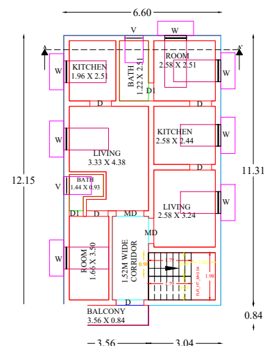
PROPOSED ST FLOOR PLAN
