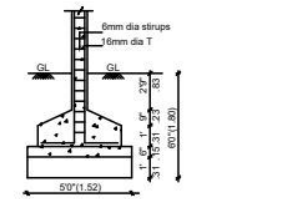
COLUMN FOUNDATION DETAIL
