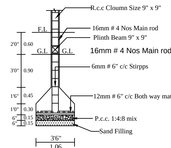
COLUMN DETIAL
