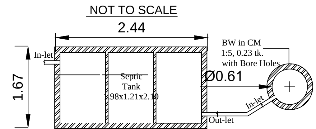
PLAN - SEPTIC TANK & SOAK PIT
