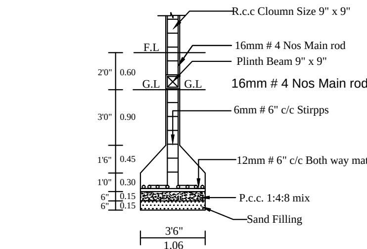
COLUMN DETIAL
