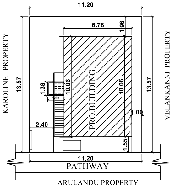
SITE PLAN
