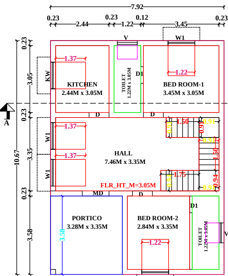
FLOOR-0 PRO.GROUND FLOOR PLAN
