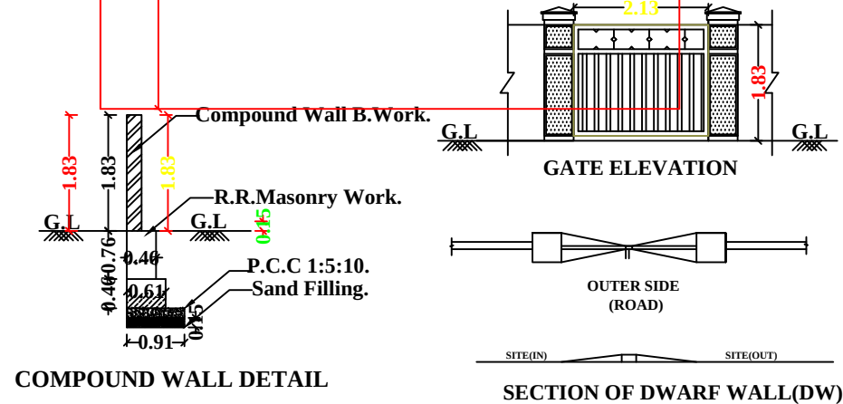
SECTION OF DWARF WALL(DW)
