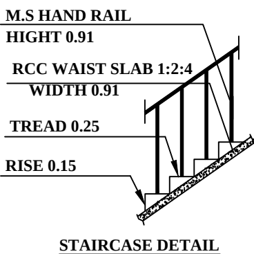
STAIRCASE DETAIL
