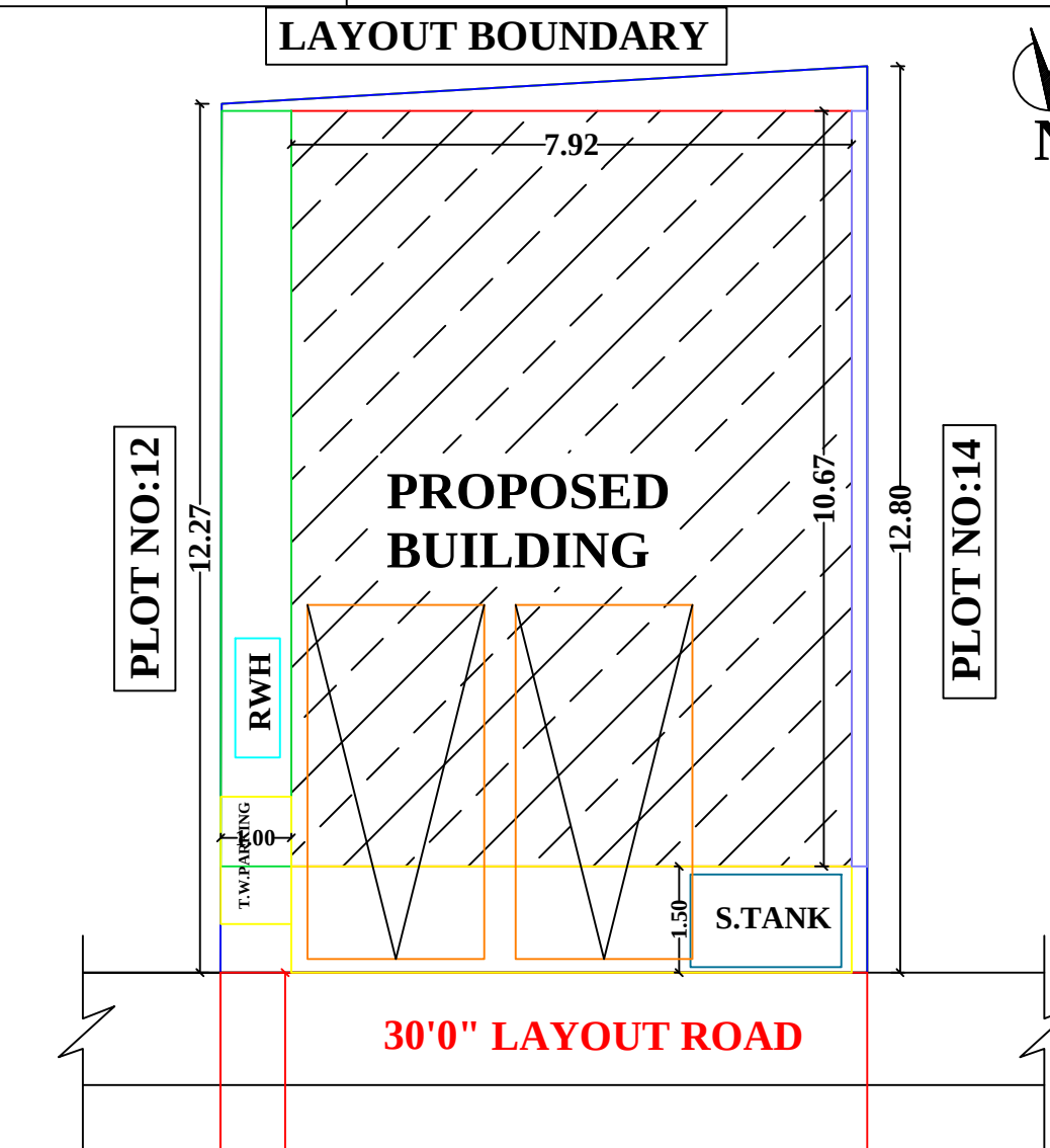
LOCATION PLAN
