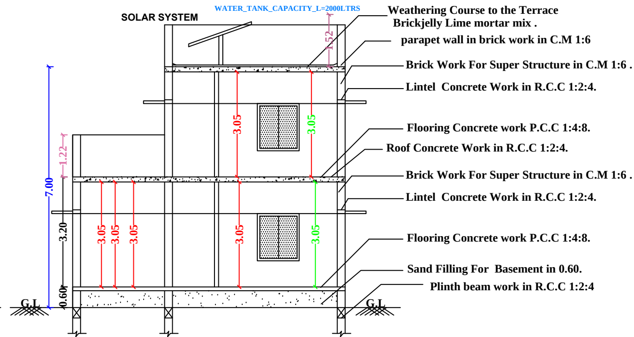
SECTION-AB
