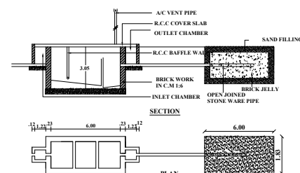
DETAILS OF SEPTIC TANK AND DISPERSION TRENCH NOT TO SCALE
