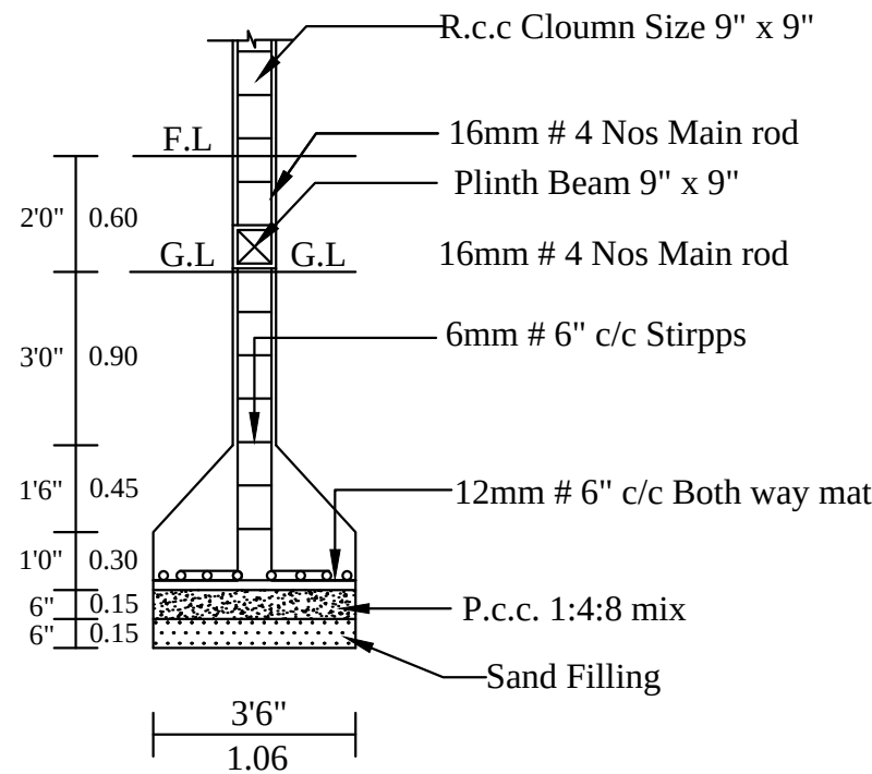
COLUMN DETIALS
