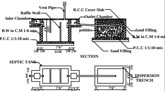
SEPTIC TANK DETAILS.
