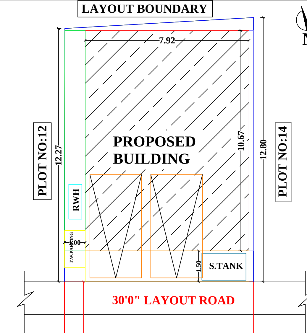
LOCATION PLAN
