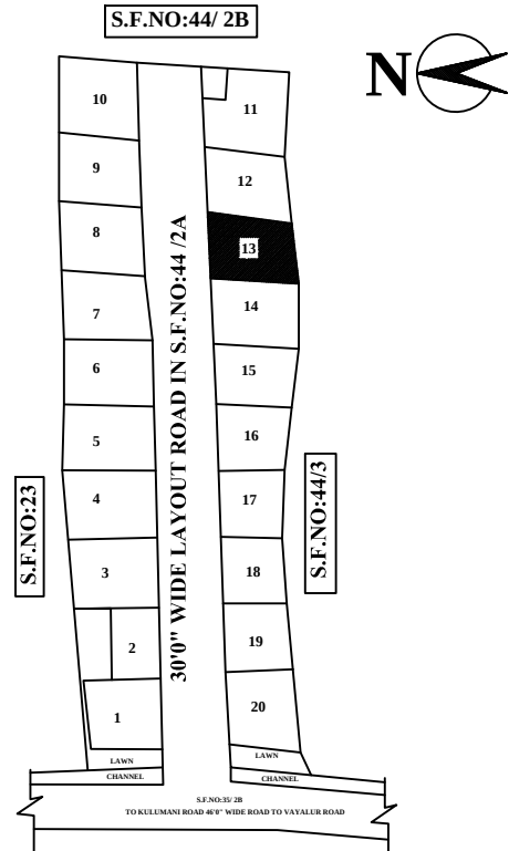
LOCATION PLAN
