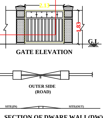
SECTION OF DWARF WALL(DW)
