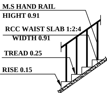
STAIRCASE DETAIL
