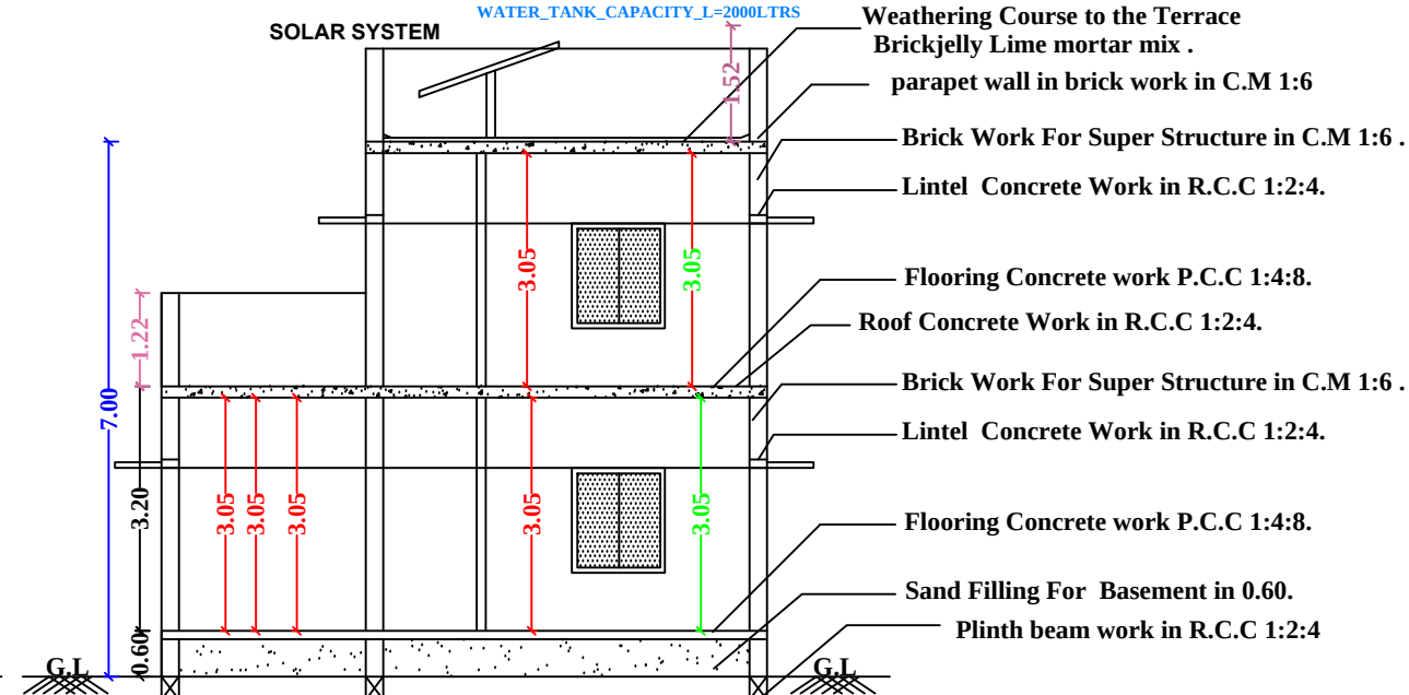
SECTION-AB
