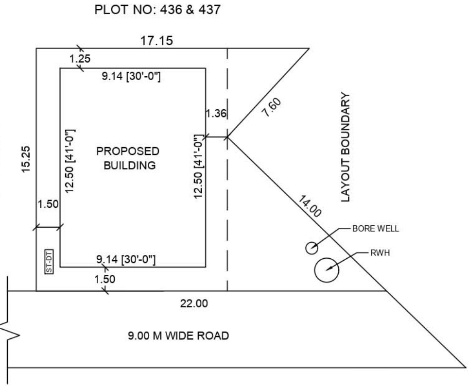
SITE PLAN
