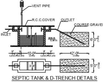
SEPTIC TANK & D-TRENCH DETAILS
