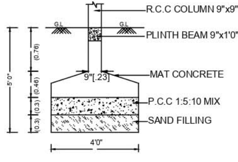
COLUMN DETAILS [NOT TO SCALE]
