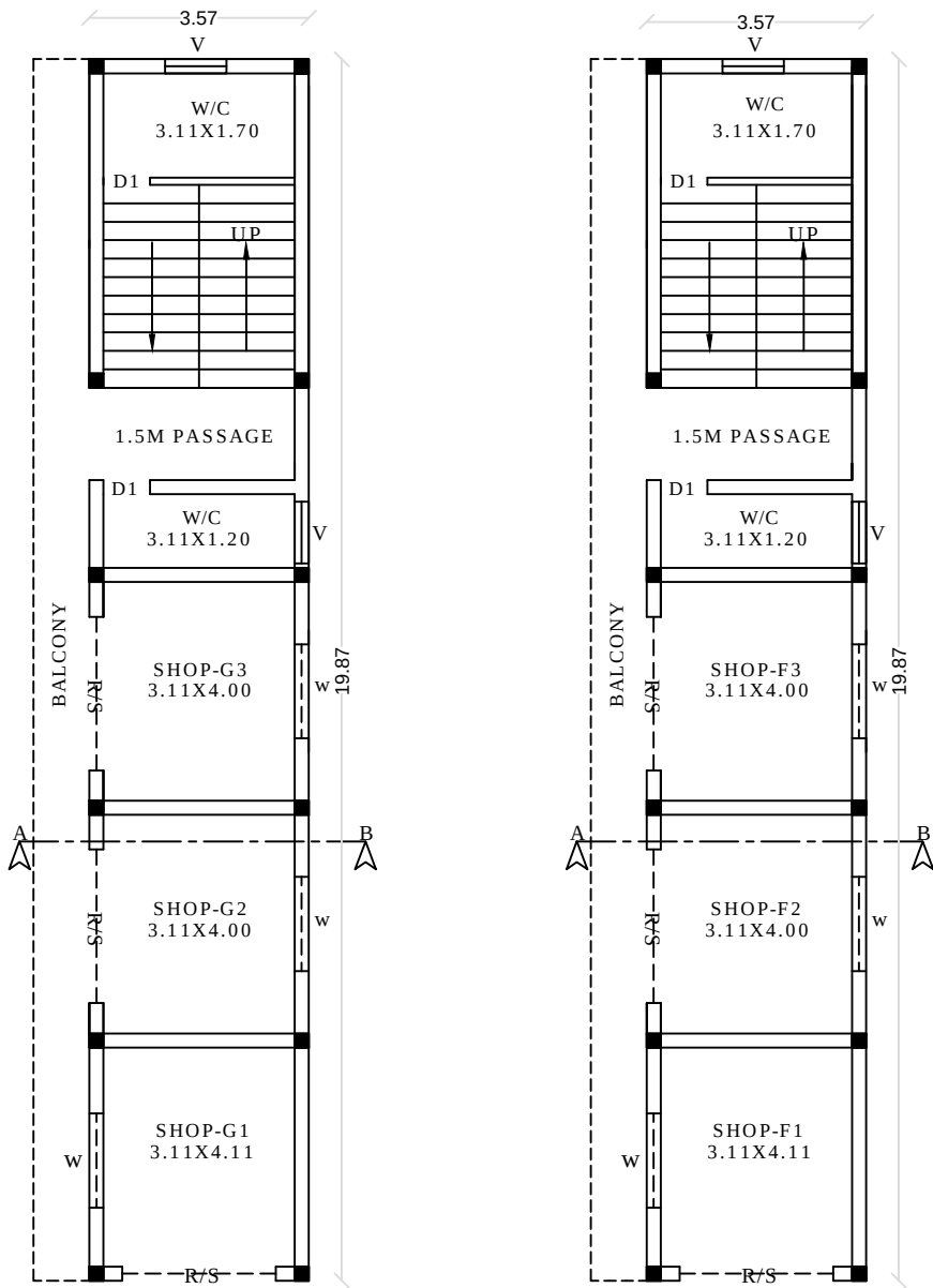
PRO.GROUND FLOOR PLAN PRO.FIRST FLOOR PLAN
