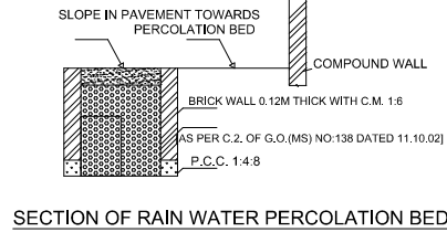
SECTION OF RAIN WATER PERCOLATION BED
