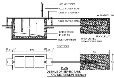
DETAILS OF SEPTIC TANK AND DISPERSION TRENCH
