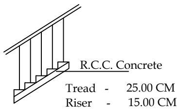
Staircase details
