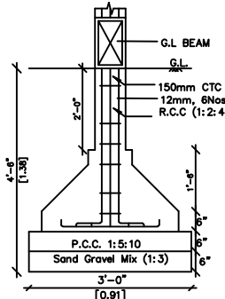
R.C.C. COLUMN FOOTING DETAILS SCALE : 1:25
