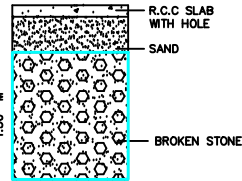
RAIN WATER HARVEST COLLECTION PIT.
