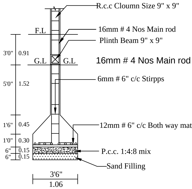
COLUMN DETIAL
