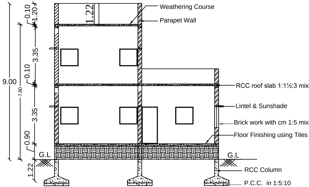
SECTION - "AB"
