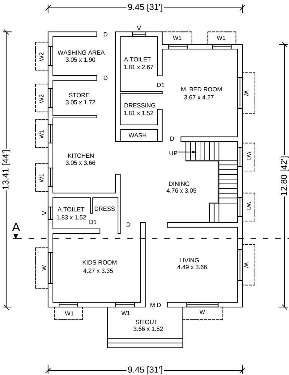
PLAN
